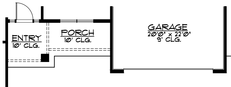
ELEVATION D
