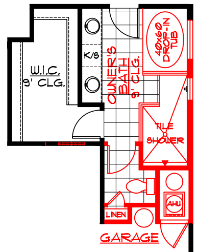
OPTIONAL OWNER'S BATH
