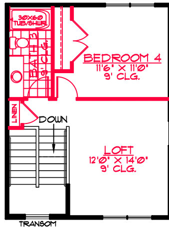
SECOND FLOOR WITH OPTIONAL BATH 3, BEDROOM 4 AND LOFT
