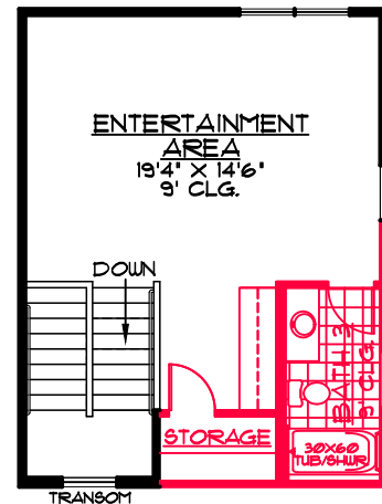
SECOND FLOOR WITH OPTIONAL BATH 3, STORAGE AND CABINETS
